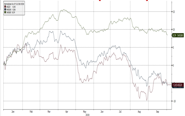
WIG20 Index (WIG20) G1111 Daily 02APR2019-02OCT2019 Copyright© 2019 Bloomberg Finance L.P. 02-Oct-2019 07:06:40
