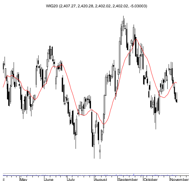
WIG20 (2,407.27, 2,420.28, 2,402.02, 2,402.02, -5.03003)
